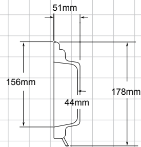
STI-6550 & STI-6560 Vista lateral
