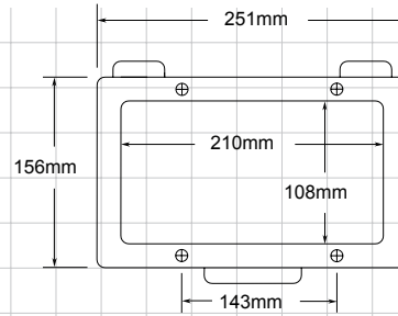
STI-6550 & STI-6560 Vista frontal
