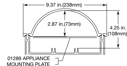
PRODUCT DIMENSIONS
